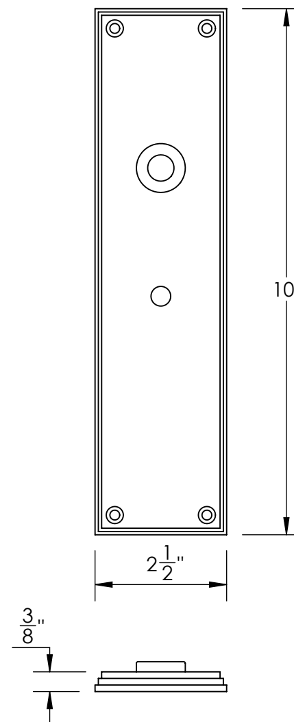
Shown above: 51893 rectangular thumbturn escutcheon plate with 48930 Lever
