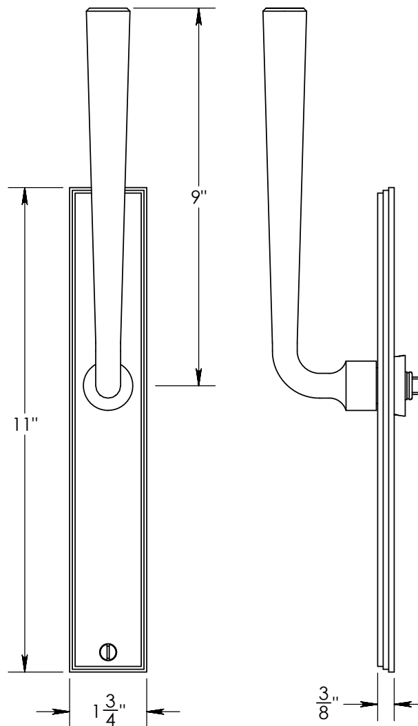
Inside Lever
