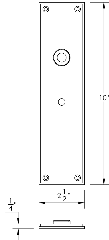
Shown above: 51693 rectangular thumbturn escutcheon plate with 48930 Lever
