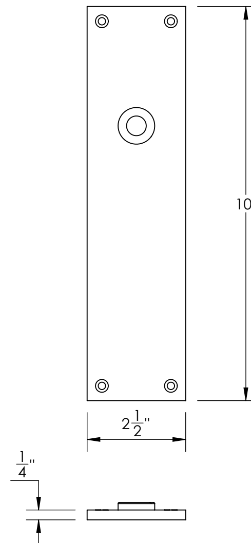
Shown above: 51433 escutcheon plate with 47134 knob
