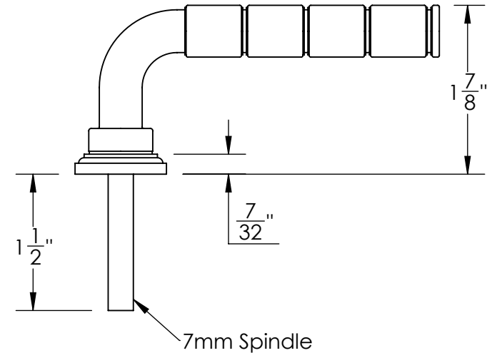
-04 stepped 1" x 2 3/8"
