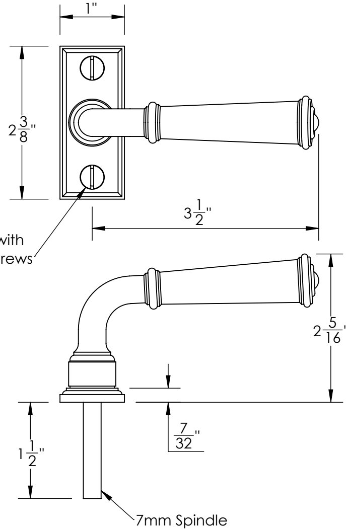
-04 stepped 1" x 2 3/8"
