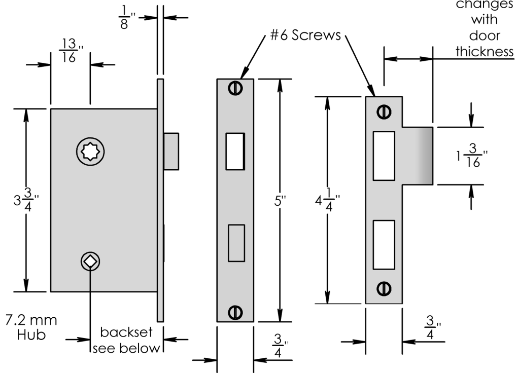
Mortise Lock 1½", 1¾", and 2" backsets available
