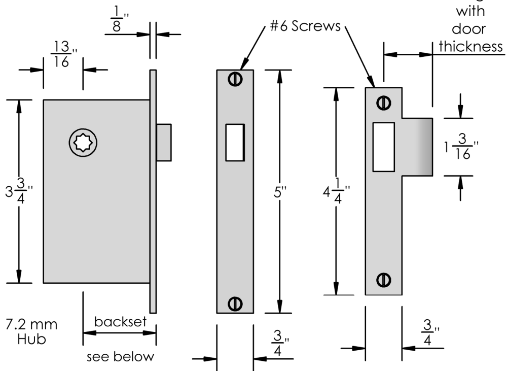
Mortise Lock 1½", 1¾", and 2" backsets available
