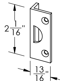
Angle Strike
