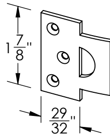
Universal Strike
